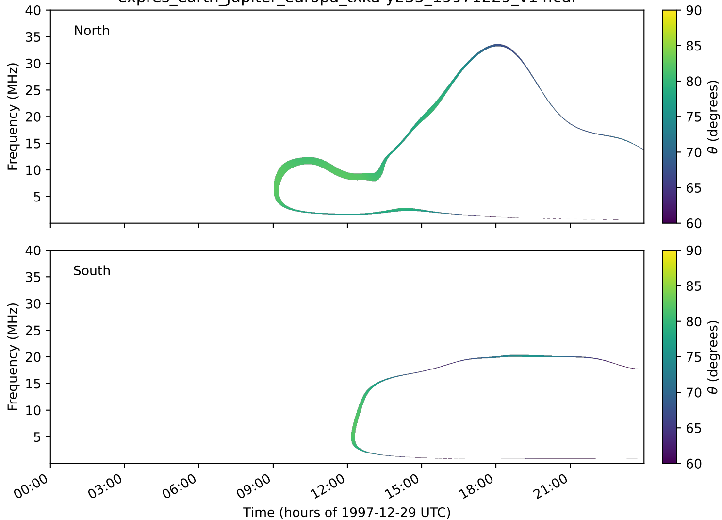
expres_earth_jupiter_europa_txka-y235_19971229_v14.cdf
