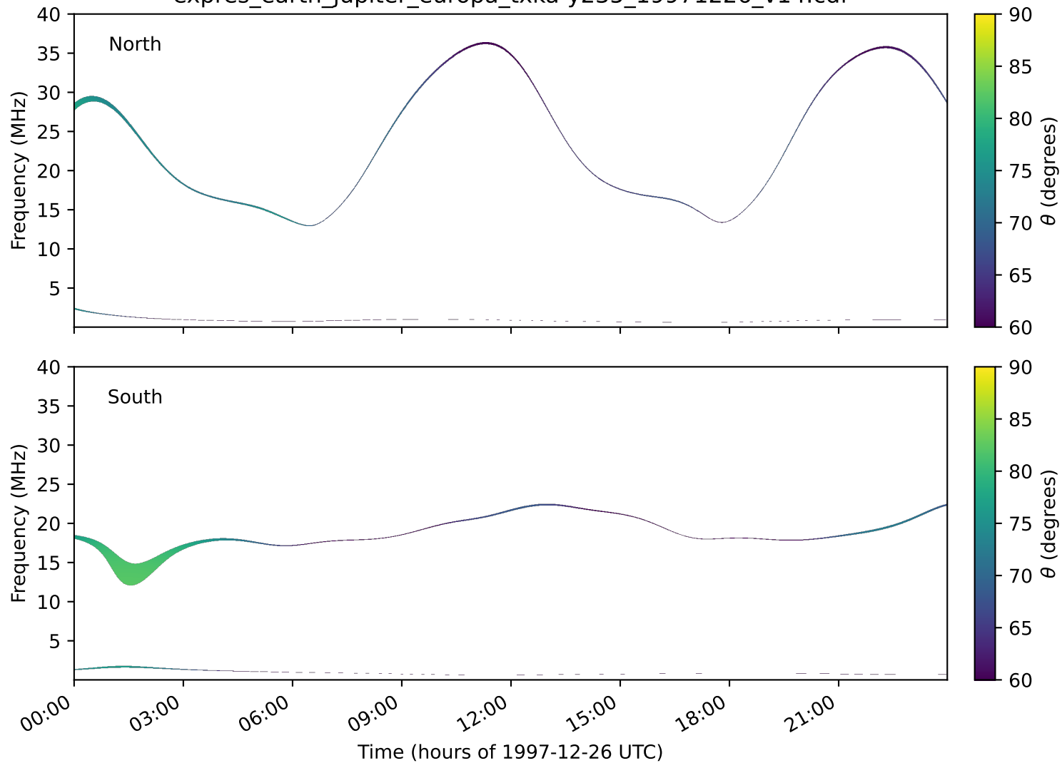
expres_earth_jupiter_europa_txka-y235_19971226_v14.cdf
