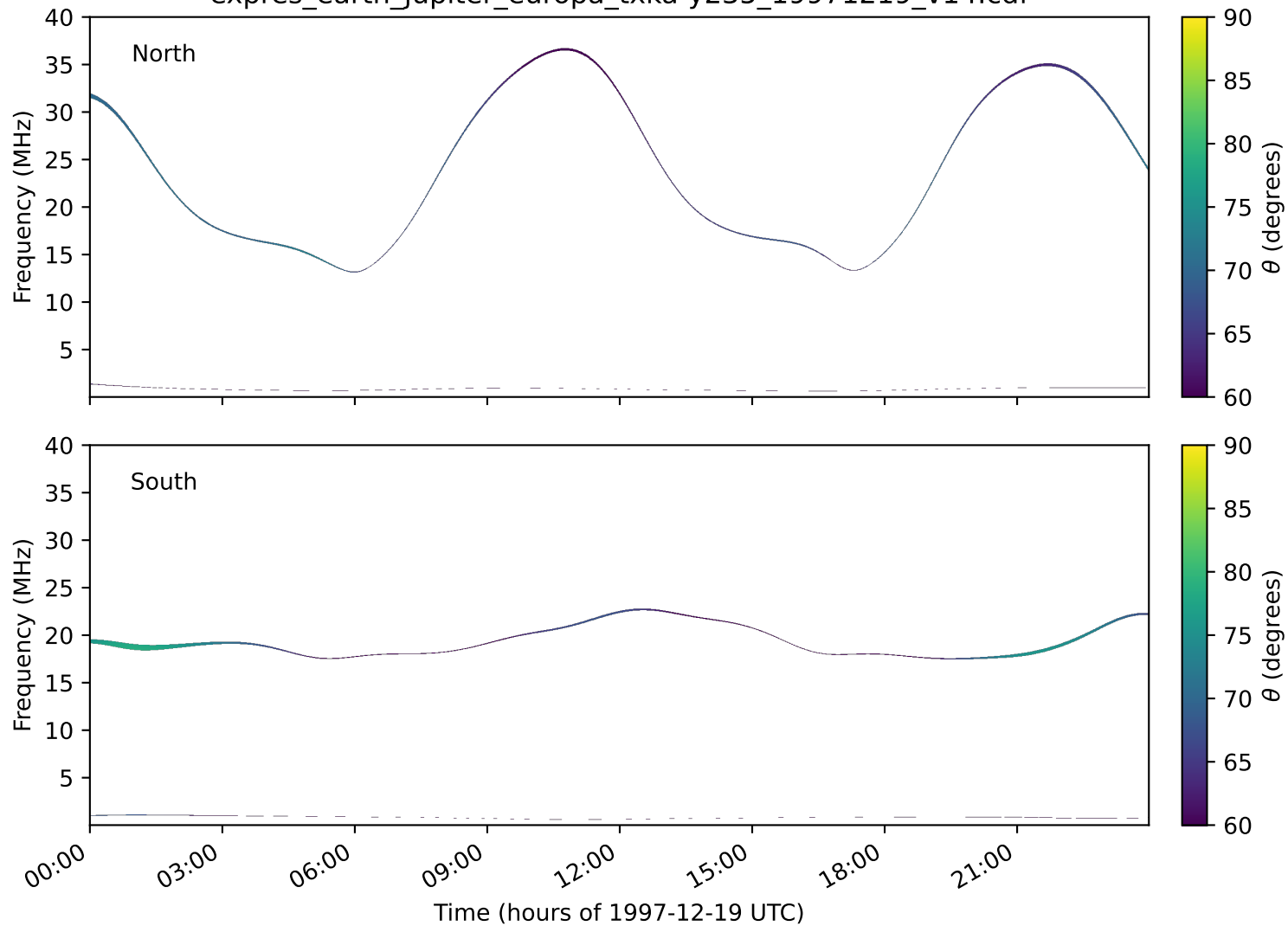
expres_earth_jupiter_europa_txka-y235_19971219_v14.cdf
