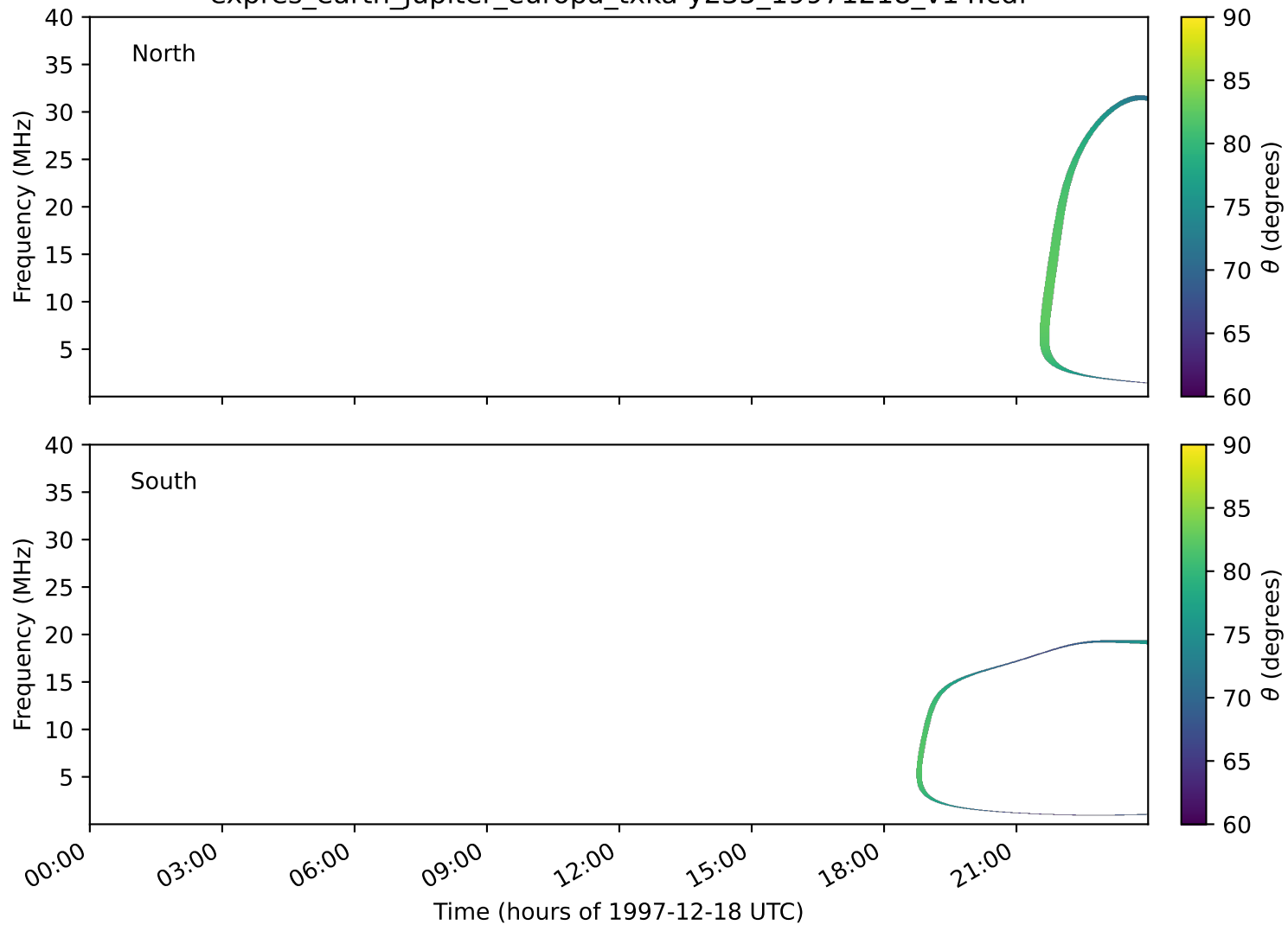
expres_earth_jupiter_europa_txka-y235_19971218_v14.cdf
