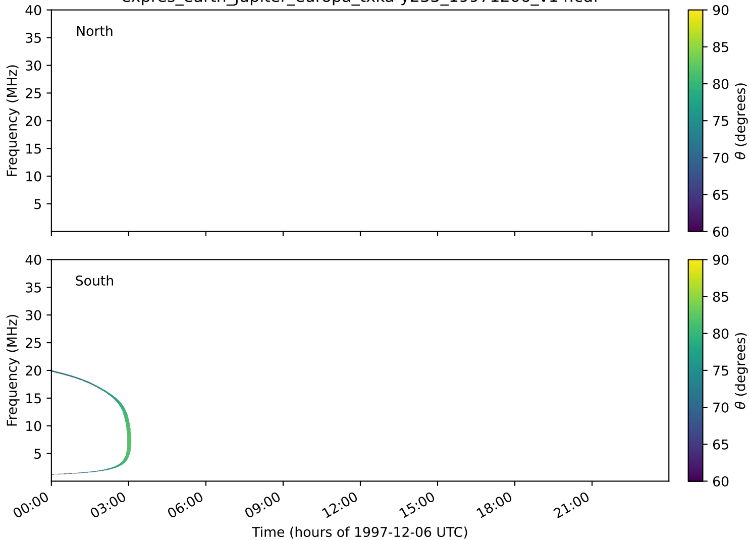
expres_earth_jupiter_europa_txka-y235_19971206_v14.cdf
