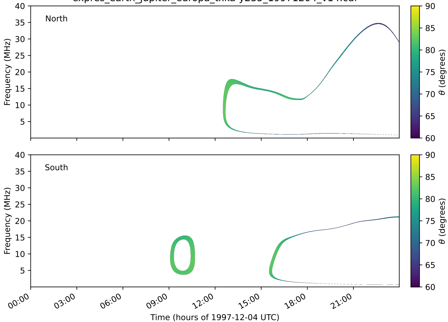
expres_earth_jupiter_europa_txka-y235_19971204_v14.cdf
