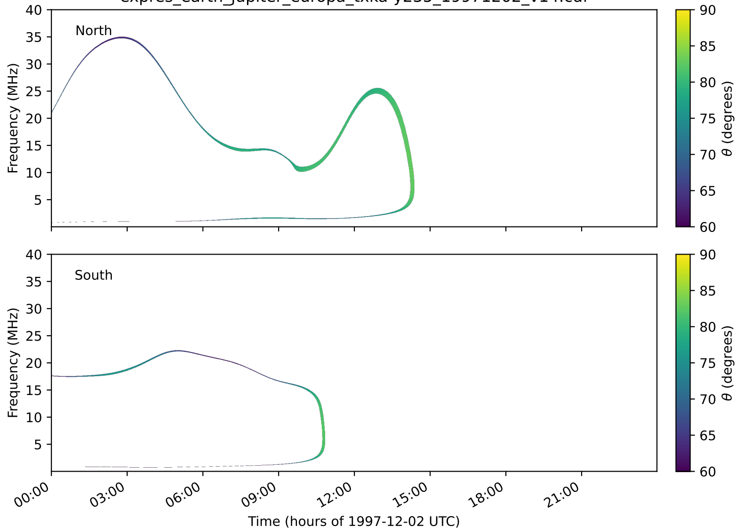
expres_earth_jupiter_europa_txka-y235_19971202_v14.cdf
