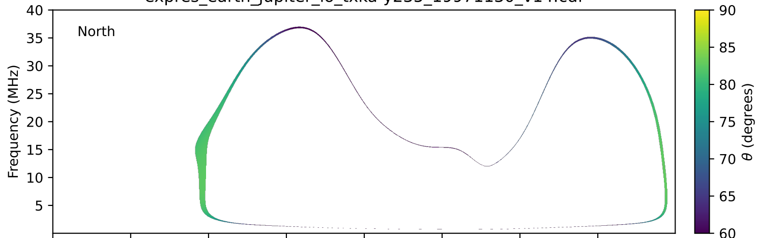
expres_earth_jupiter_io_txka-y235_19971130_v14.cdf
