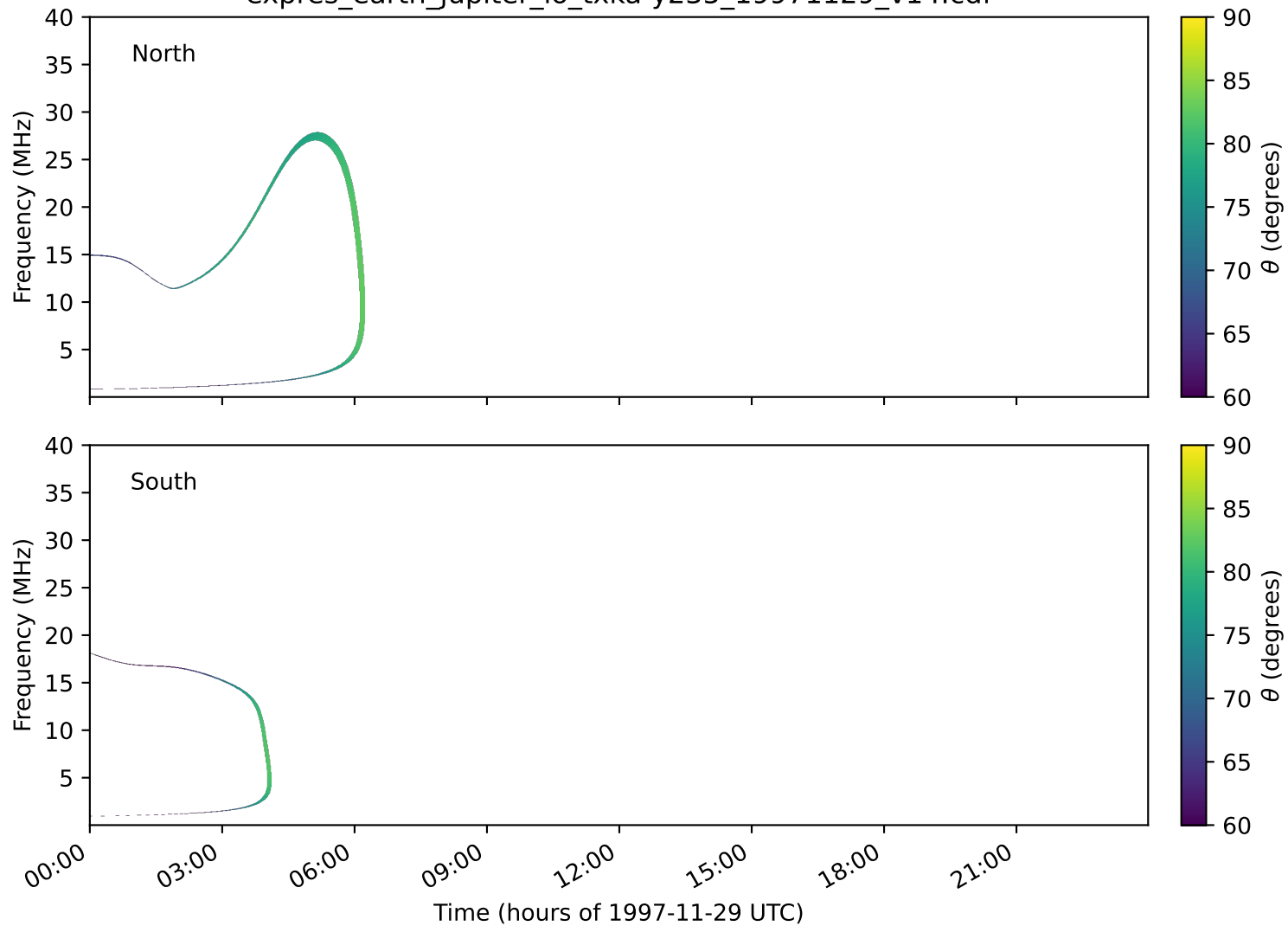
expres_earth_jupiter_io_txka-y235_19971129_v14.cdf
