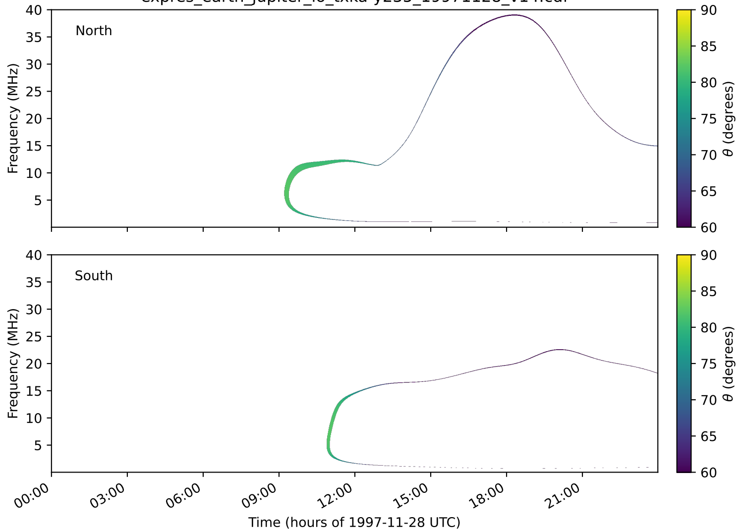
expres_earth_jupiter_io_txka-y235_19971128_v14.cdf
