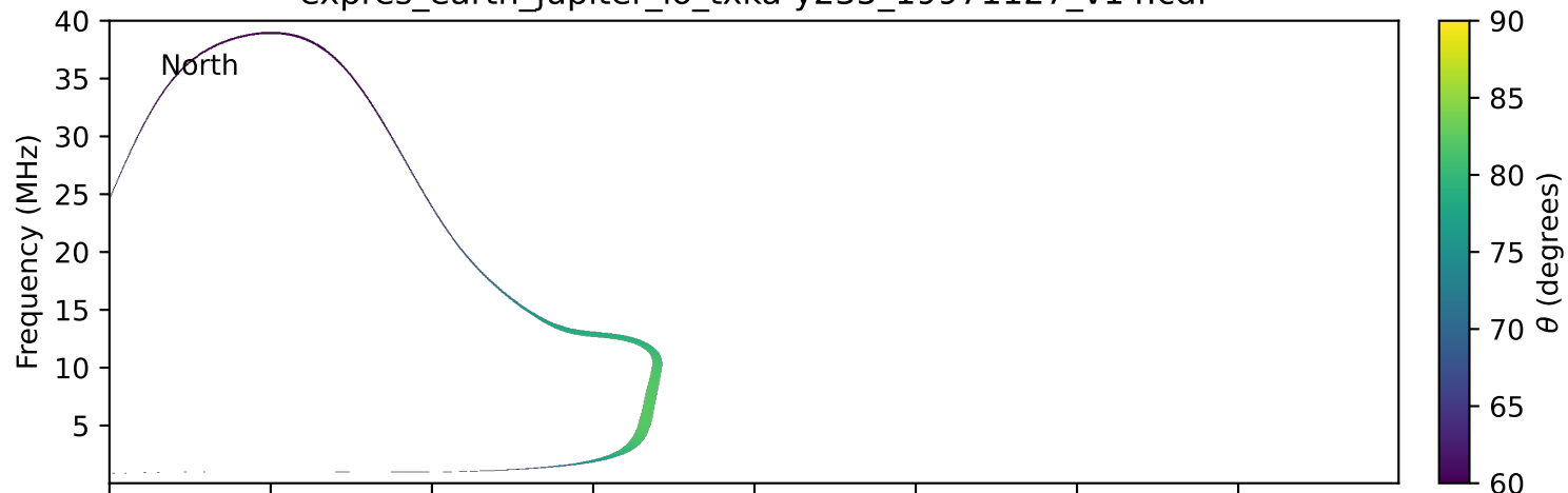
expres_earth_jupiter_io_txka-y235_19971127_v14.cdf
