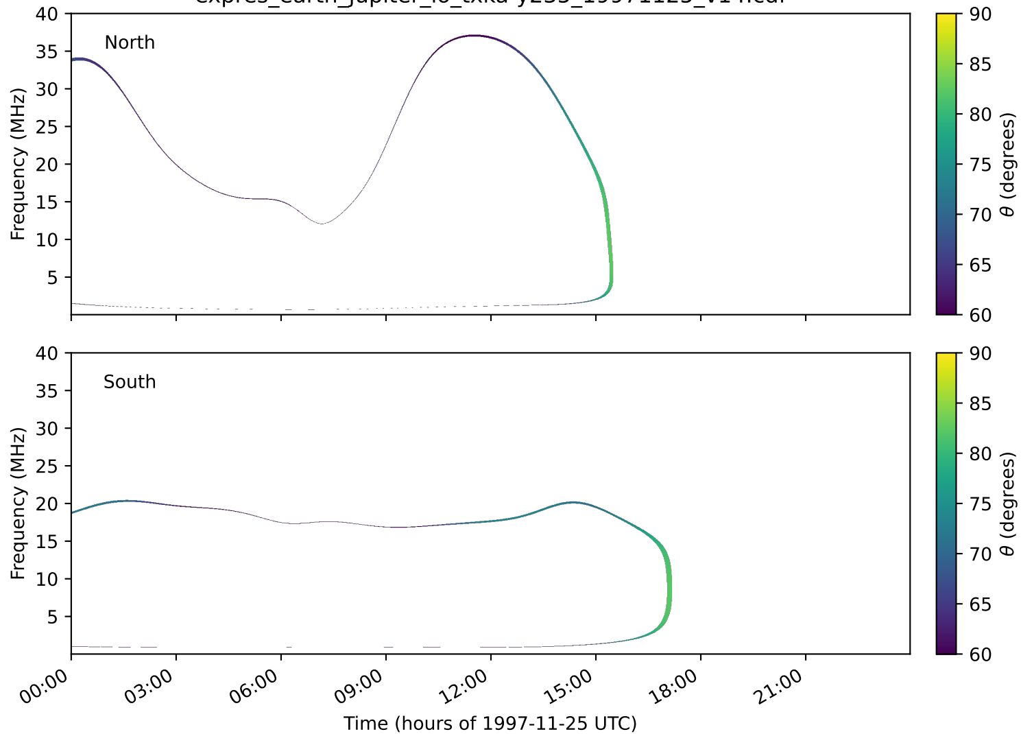
expres_earth_jupiter_io_txka-y235_19971125_v14.cdf
