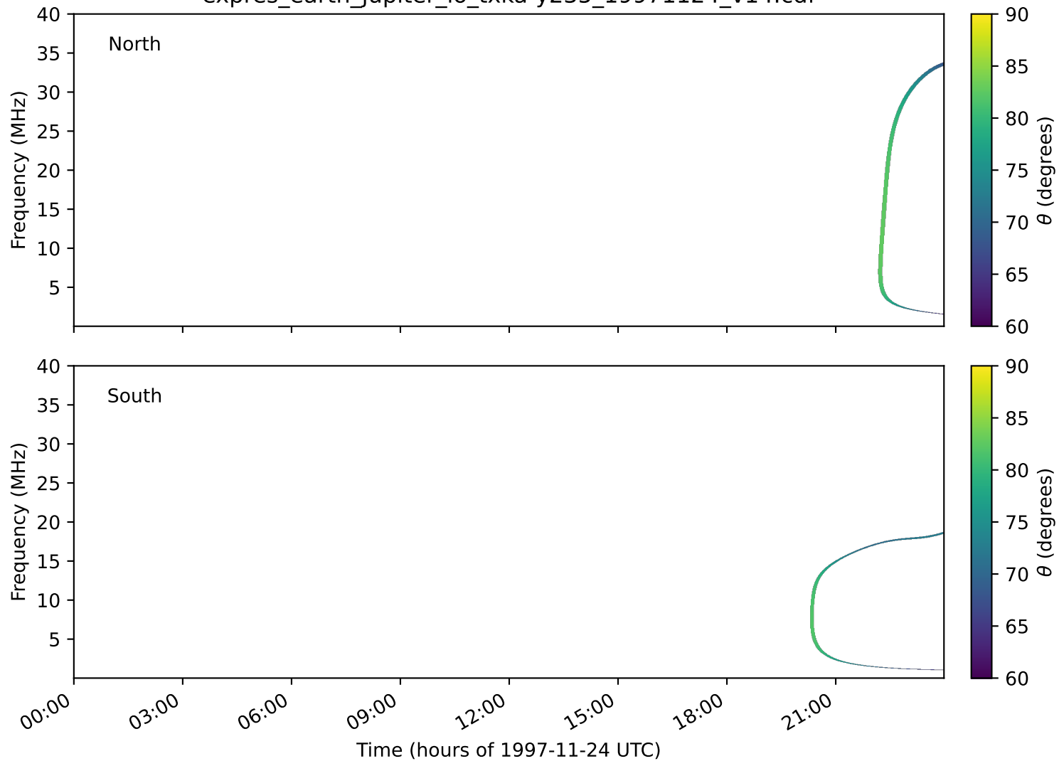
expres_earth_jupiter_io_txka-y235_19971124_v14.cdf
