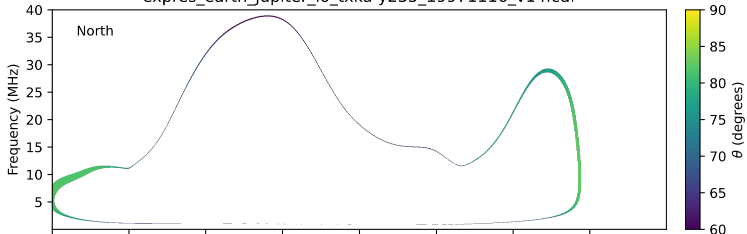
expres_earth_jupiter_io_txka-y235_19971116_v14.cdf
