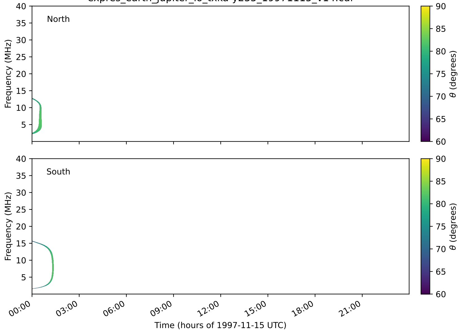
expres_earth_jupiter_io_txka-y235_19971115_v14.cdf
