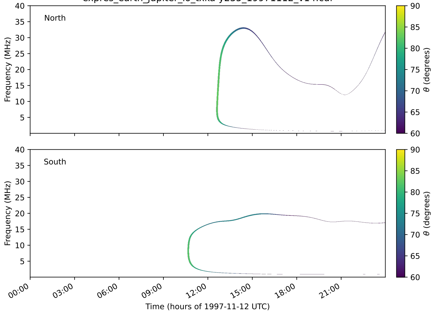
expres_earth_jupiter_io_txka-y235_19971112_v14.cdf
