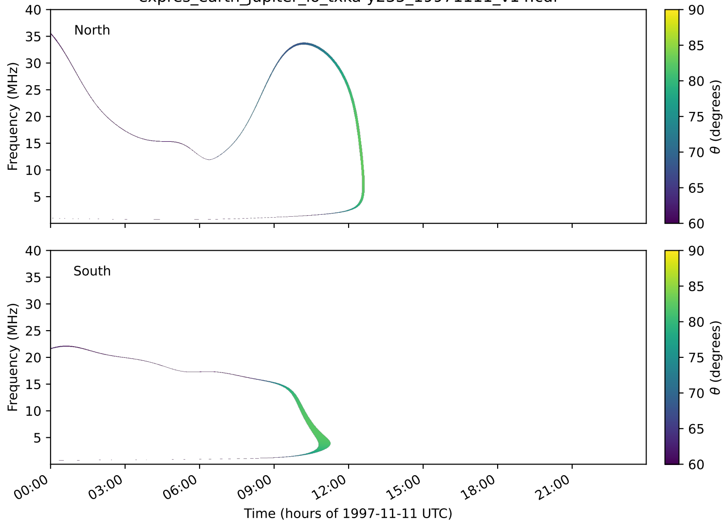
expres_earth_jupiter_io_txka-y235_19971111_v14.cdf
