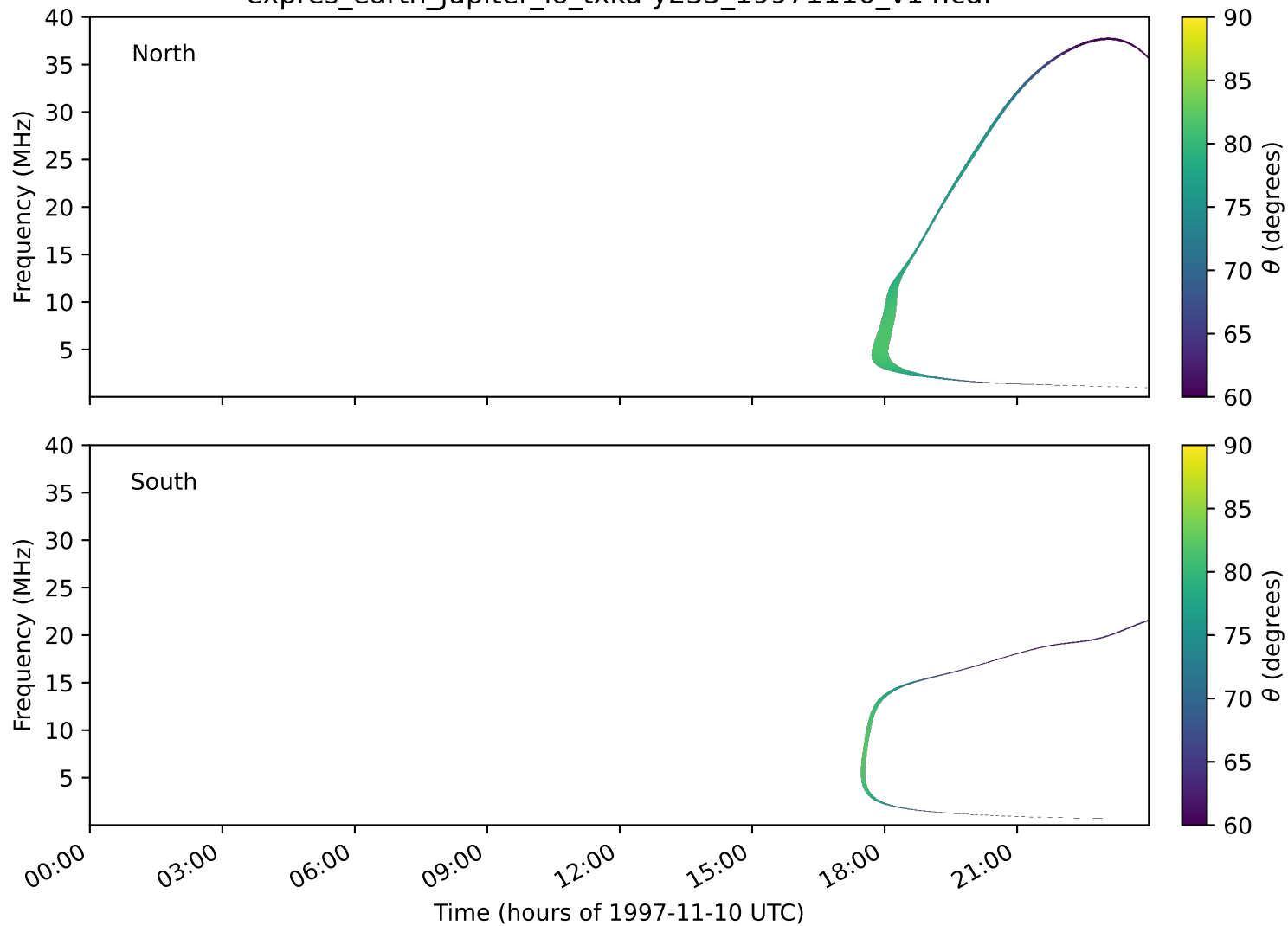
expres_earth_jupiter_io_txka-y235_19971110_v14.cdf
