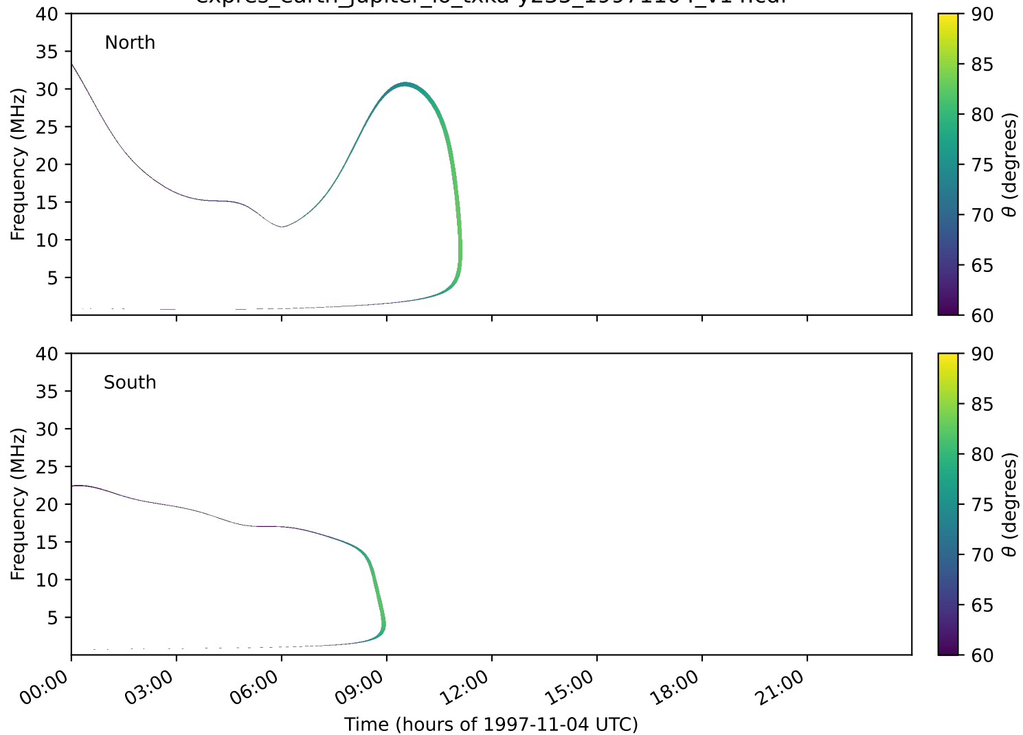
expres_earth_jupiter_io_txka-y235_19971104_v14.cdf
