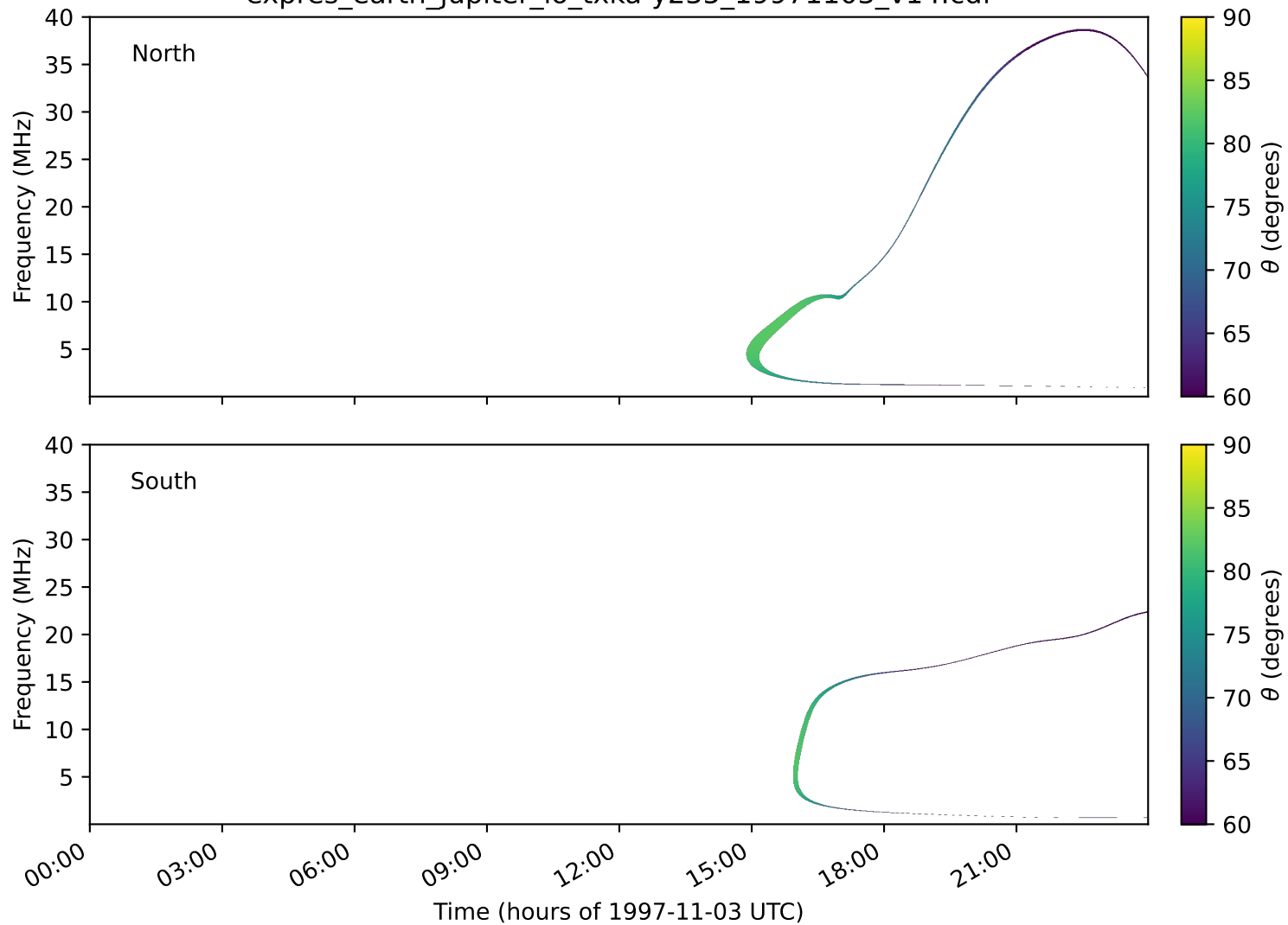
expres_earth_jupiter_io_txka-y235_19971103_v14.cdf
