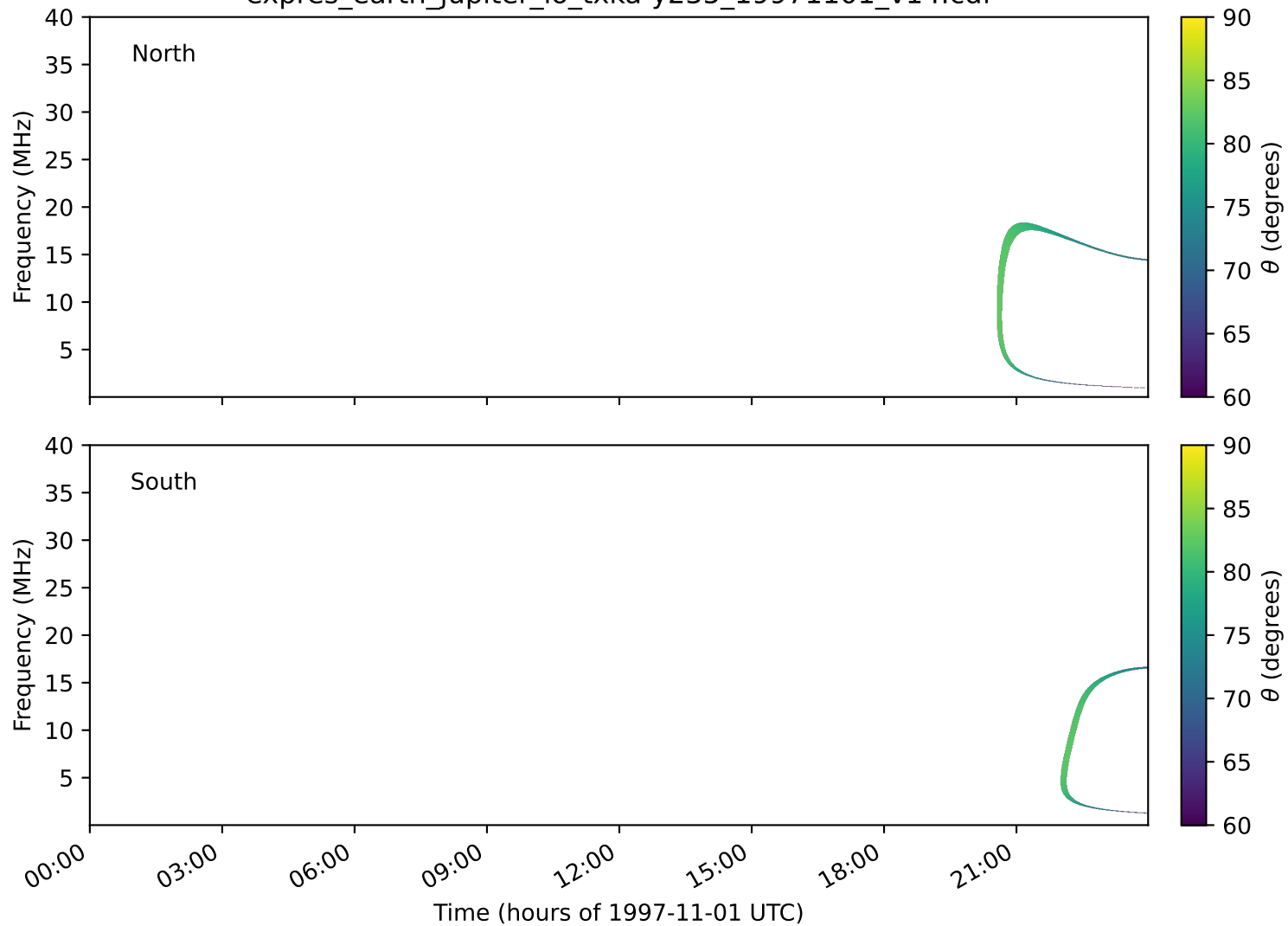
expres_earth_jupiter_io_txka-y235_19971101_v14.cdf
