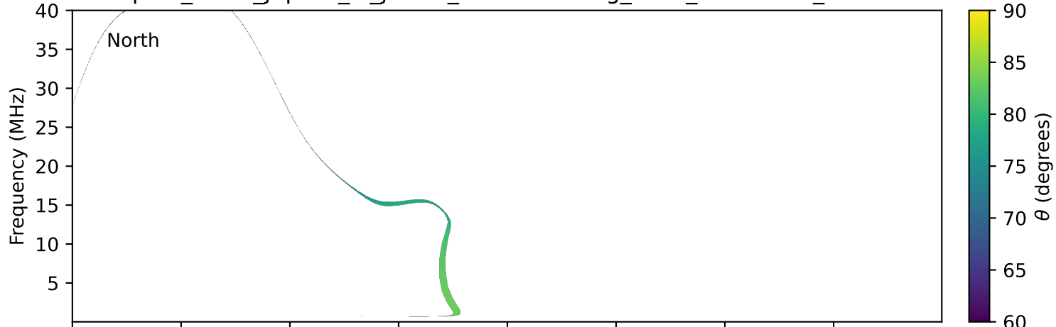
expres_earth_jupiter_io_jrm33_lossc-wid1deg_3kev_19971127_v11.cdf
