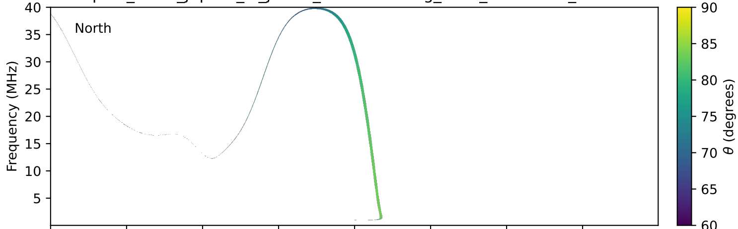
expres_earth_jupiter_io_jrm33_lossc-wid1deg_3kev_19971111_v11.cdf
