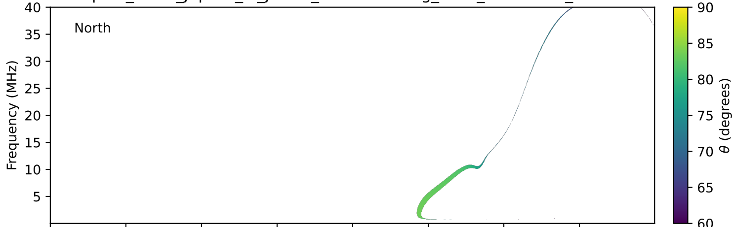
expres_earth_jupiter_io_jrm33_lossc-wid1deg_3kev_19971103_v11.cdf
