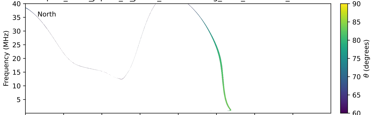
expres_earth_jupiter_io_jrm09_lossc-wid1deg_3kev_19971125_v11.cdf
