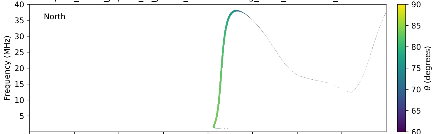
expres_earth_jupiter_io_jrm09_lossc-wid1deg_3kev_19971112_v11.cdf
