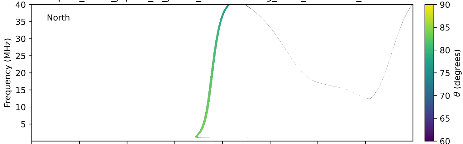
expres_earth_jupiter_io_jrm09_lossc-wid1deg_3kev_19971105_v11.cdf
