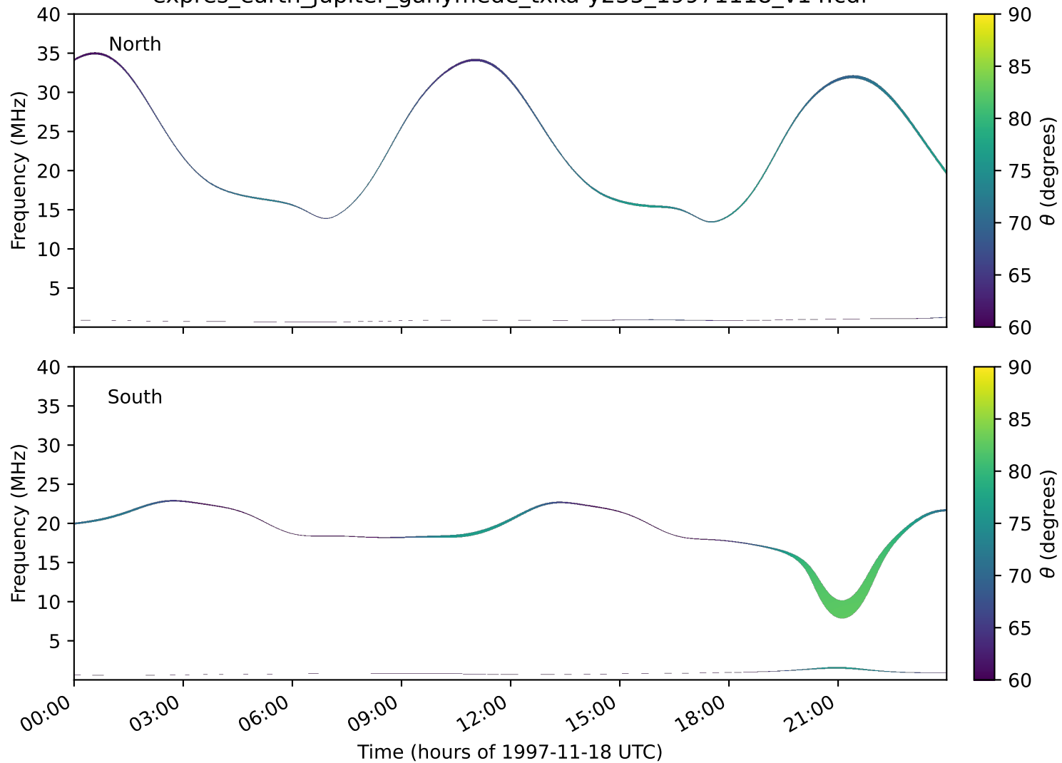
expres_earth_jupiter_ganymede_txka-y235_19971118_v14.cdf
