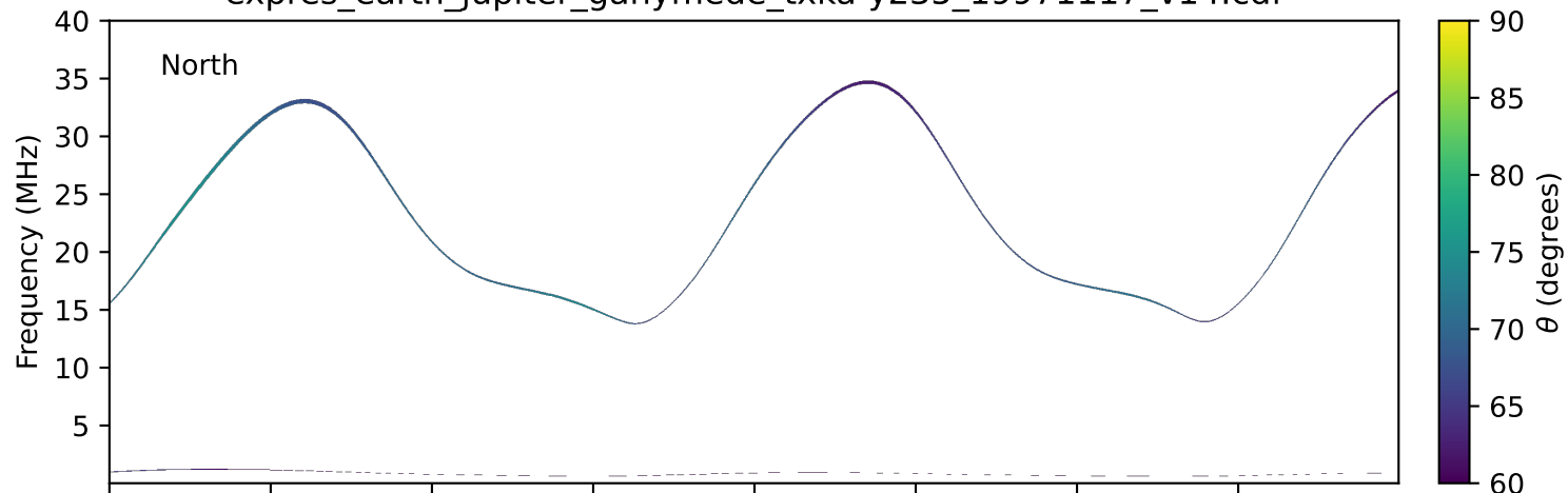
expres_earth_jupiter_ganymede_txka-y235_19971117_v14.cdf
