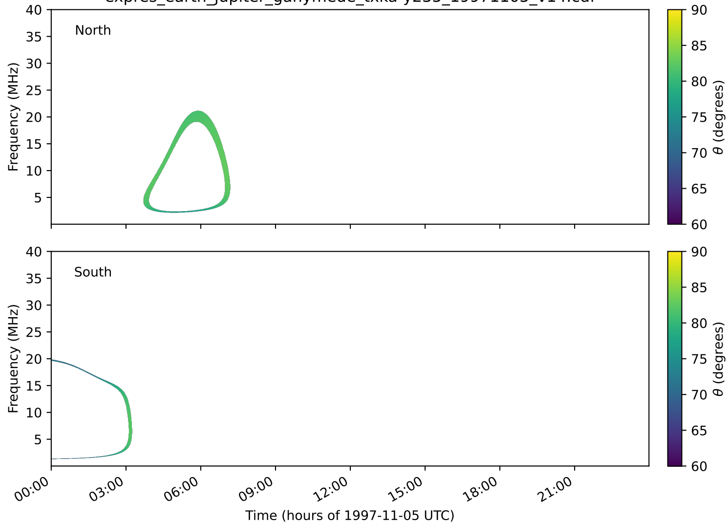
expres_earth_jupiter_ganymede_txka-y235_19971105_v14.cdf
