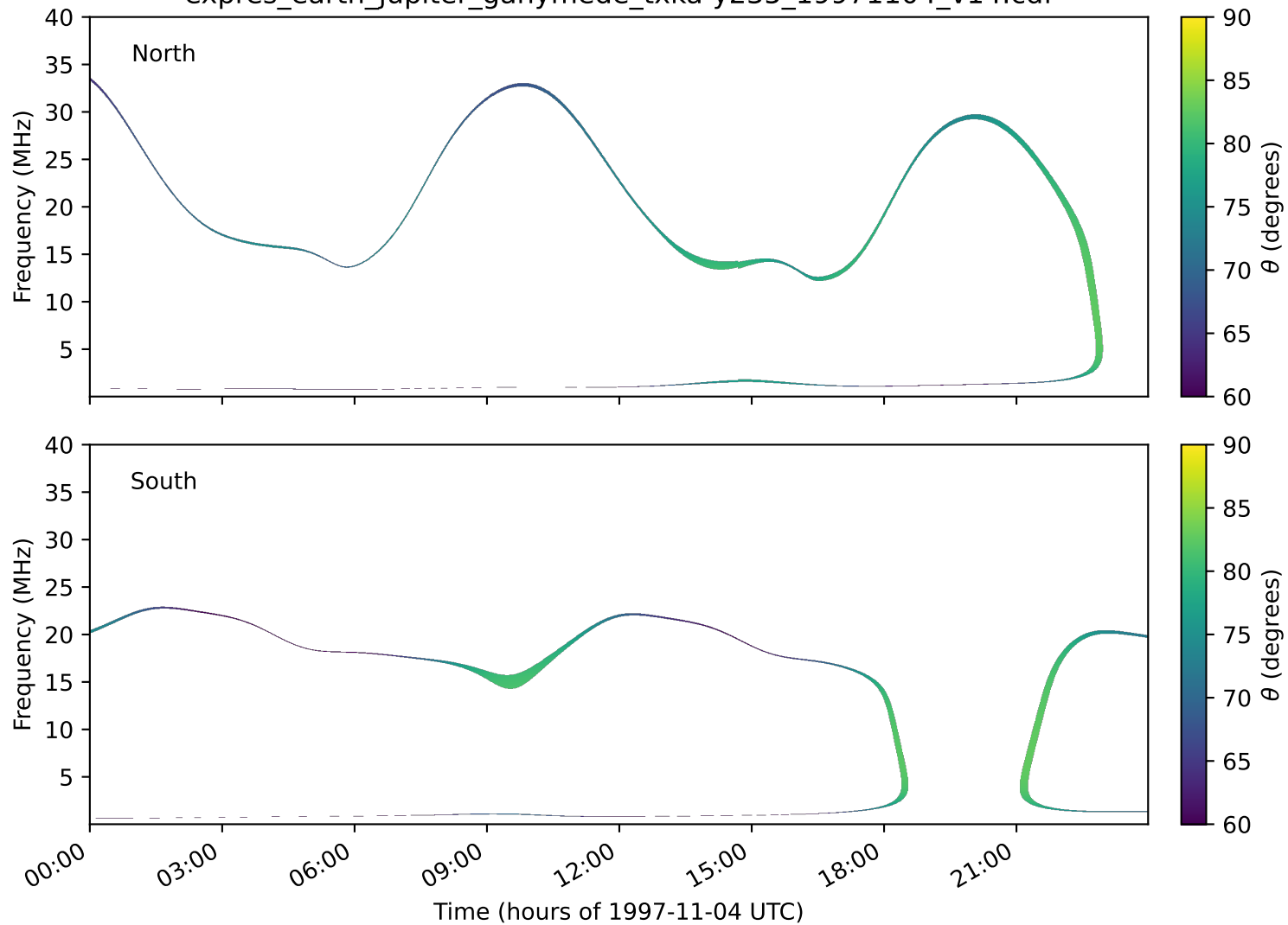
expres_earth_jupiter_ganymede_txka-y235_19971104_v14.cdf
