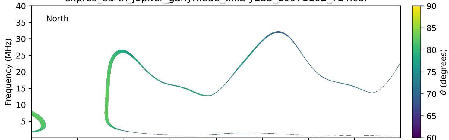
expres_earth_jupiter_ganymede_txka-y235_19971102_v14.cdf
