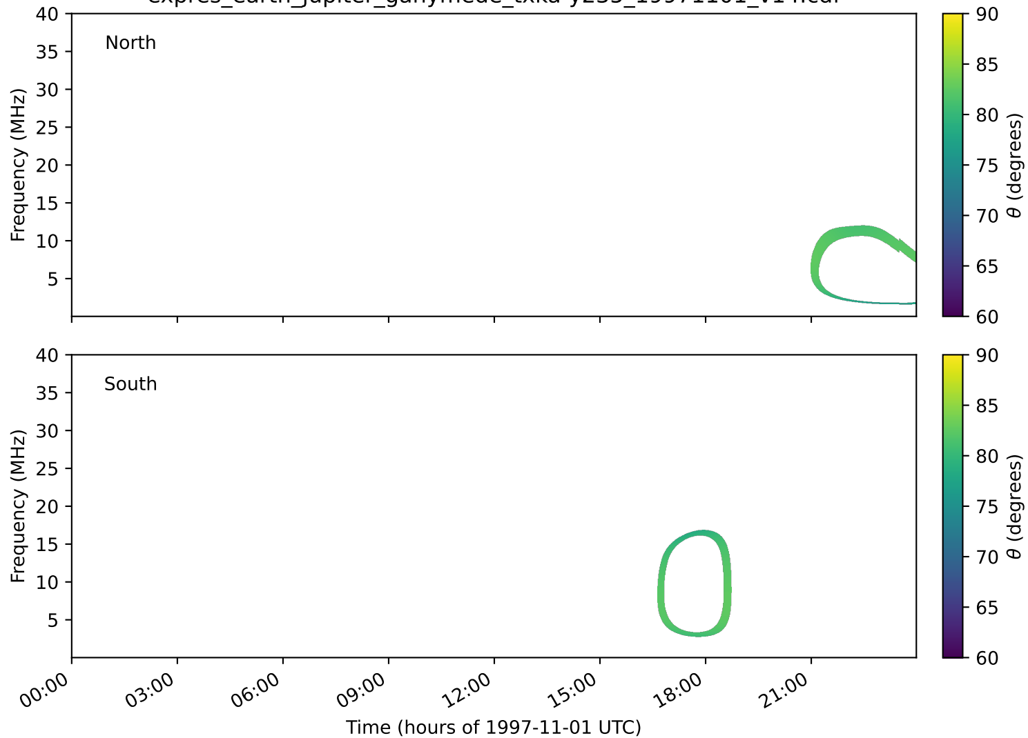
expres_earth_jupiter_ganymede_txka-y235_19971101_v14.cdf
