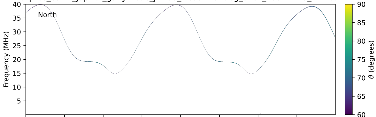
expres_earth_jupiter_ganymede_jrm33_lossc-wid1deg_3kev_19971125_v11.cdf
