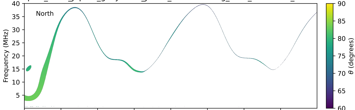
expres_earth_jupiter_ganymede_jrm33_lossc-wid1deg_3kev_19971124_v11.cdf
