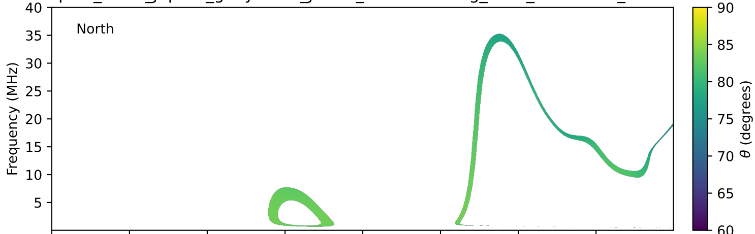
expres_earth_jupiter_ganymede_jrm33_lossc-wid1deg_3kev_19971116_v11.cdf
