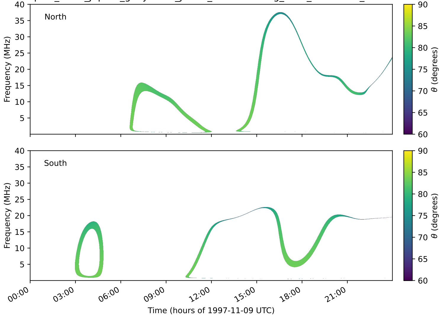
expres_earth_jupiter_ganymede_jrm33_lossc-wid1deg_3kev_19971109_v11.cdf
