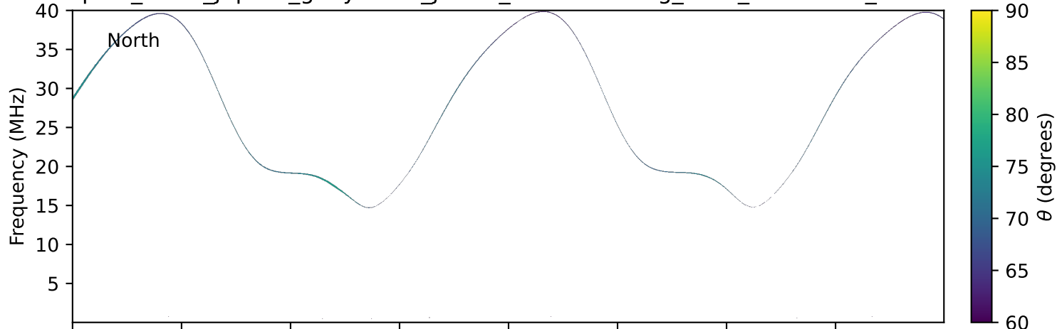
expres_earth_jupiter_ganymede_jrm33_lossc-wid1deg_3kev_19971103_v11.cdf
