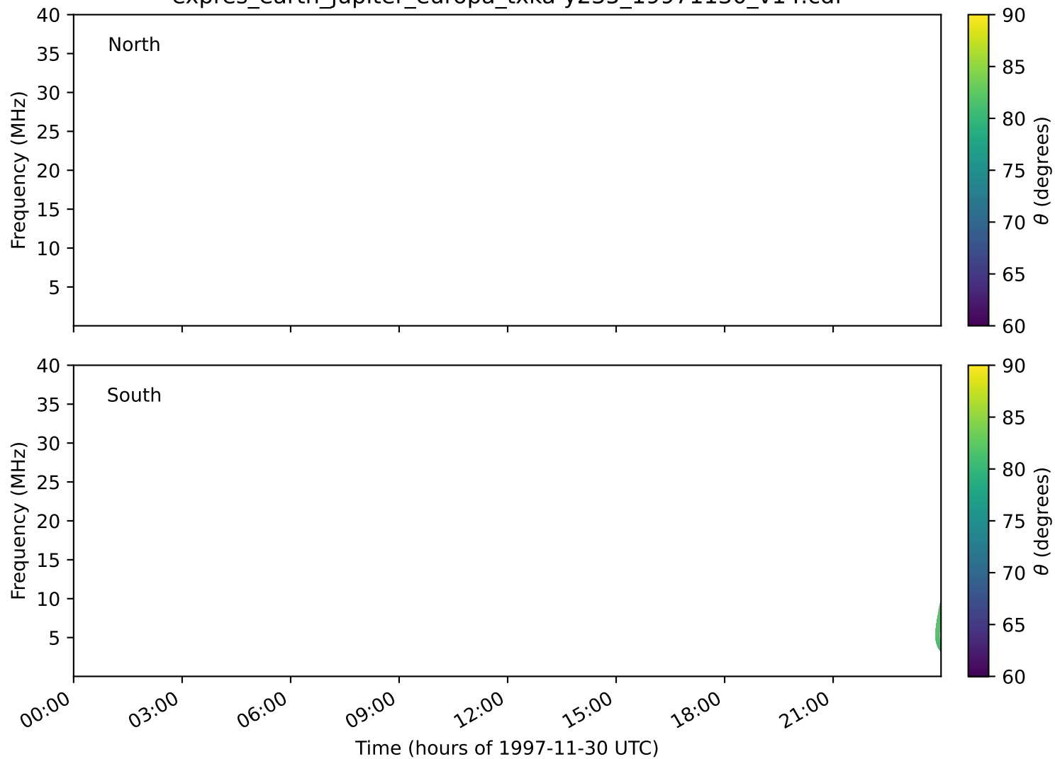
expres_earth_jupiter_europa_txka-y235_19971130_v14.cdf
