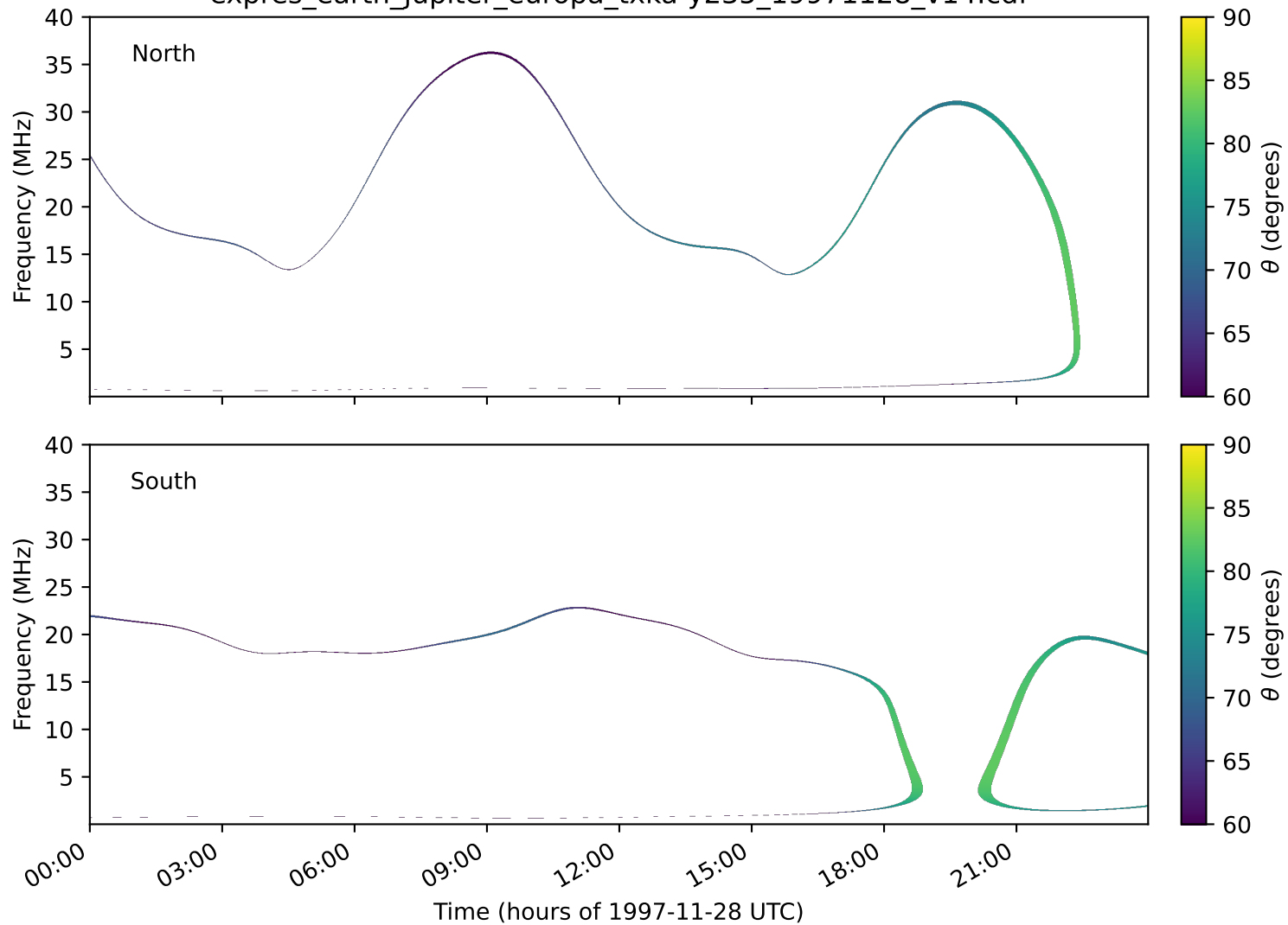
expres_earth_jupiter_europa_txka-y235_19971128_v14.cdf
