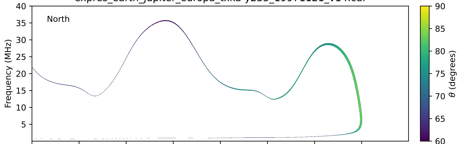
expres_earth_jupiter_europa_txka-y235_19971121_v14.cdf
