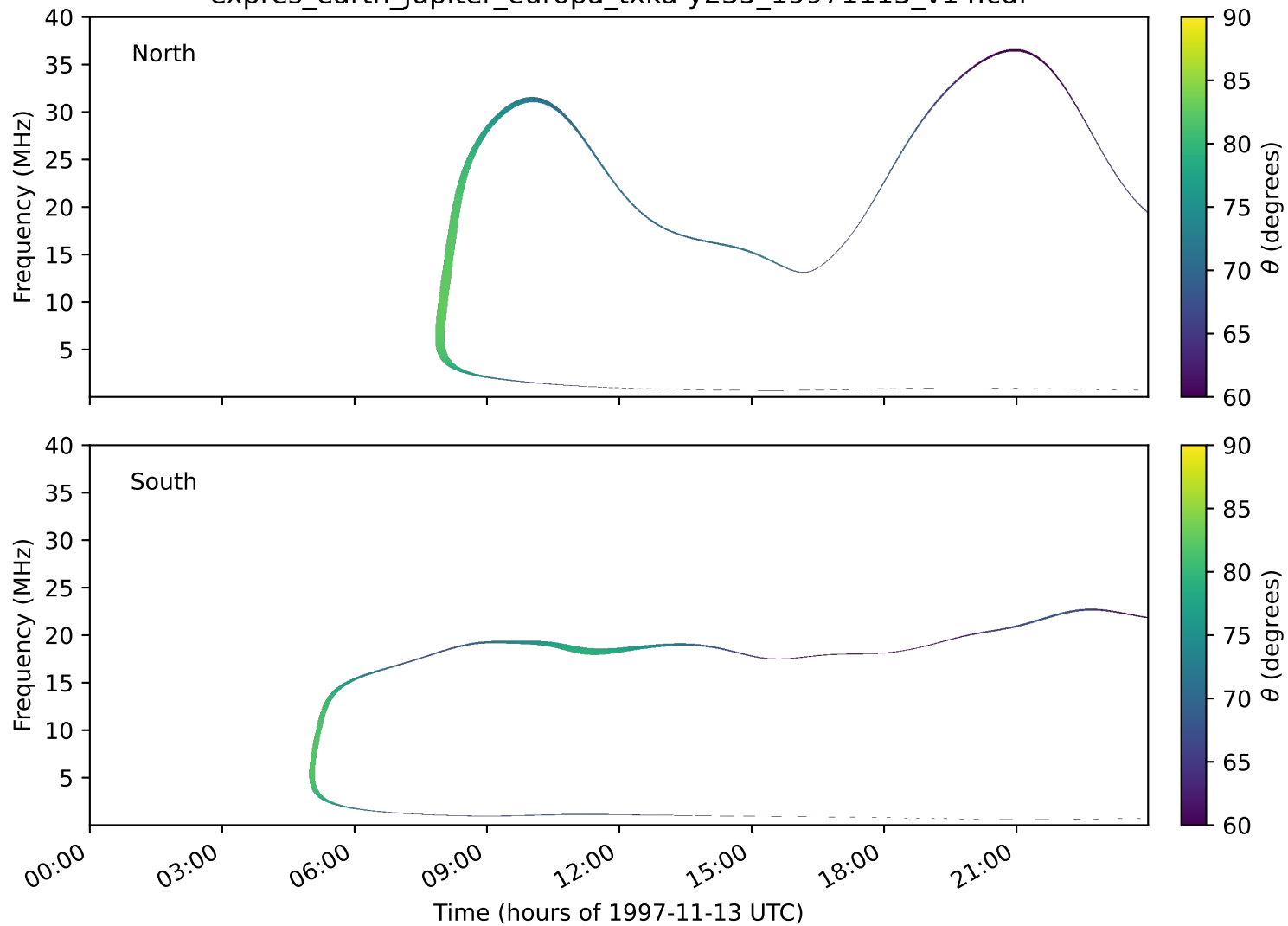
expres_earth_jupiter_europa_txka-y235_19971113_v14.cdf
