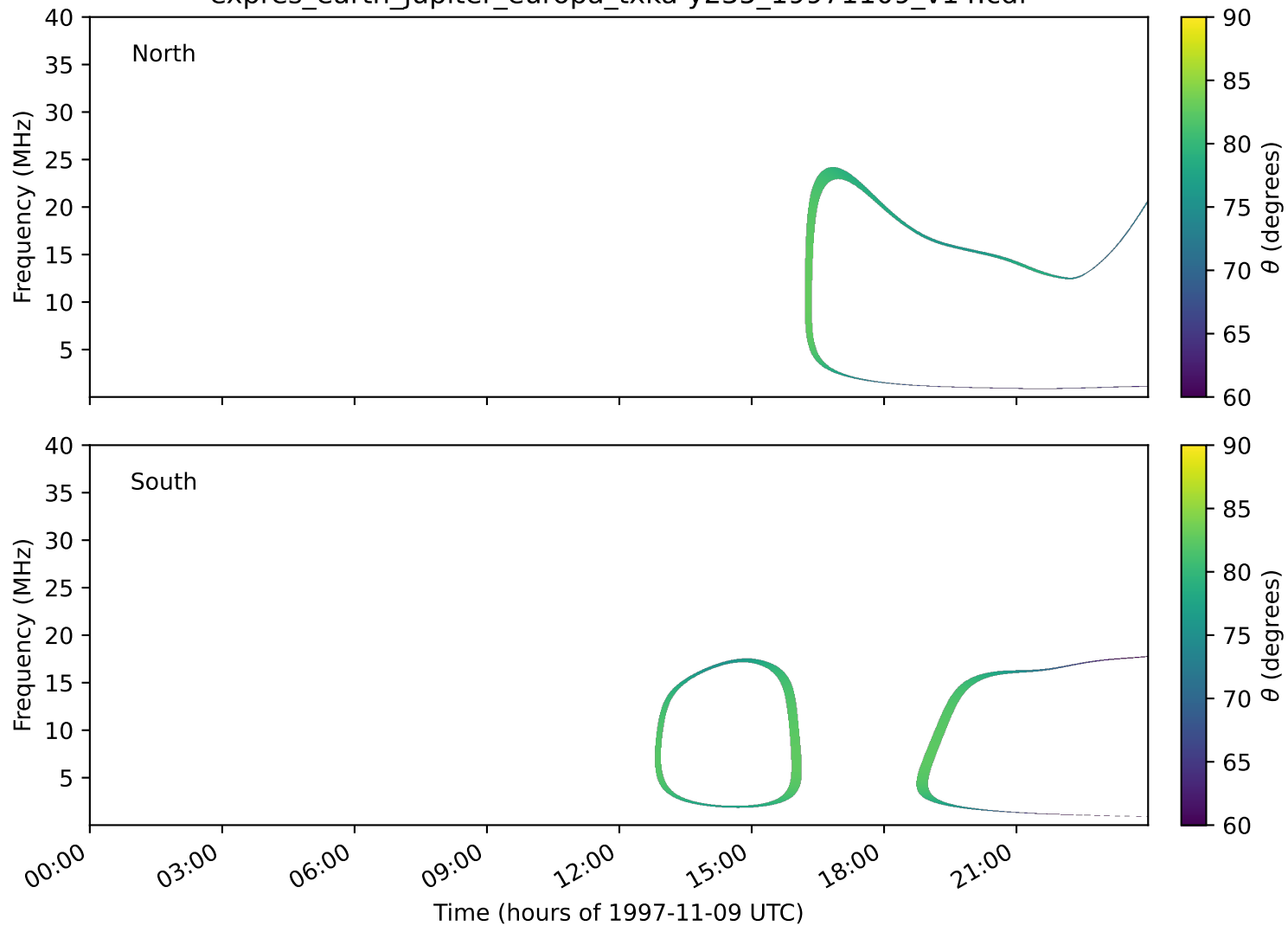
expres_earth_jupiter_europa_txka-y235_19971109_v14.cdf
