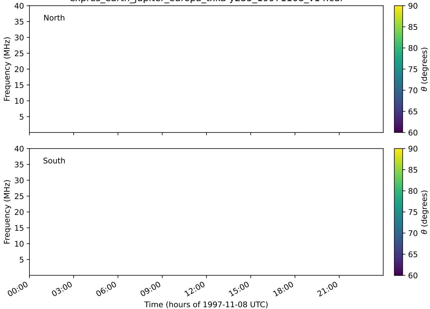
expres_earth_jupiter_europa_txka-y235_19971108_v14.cdf
