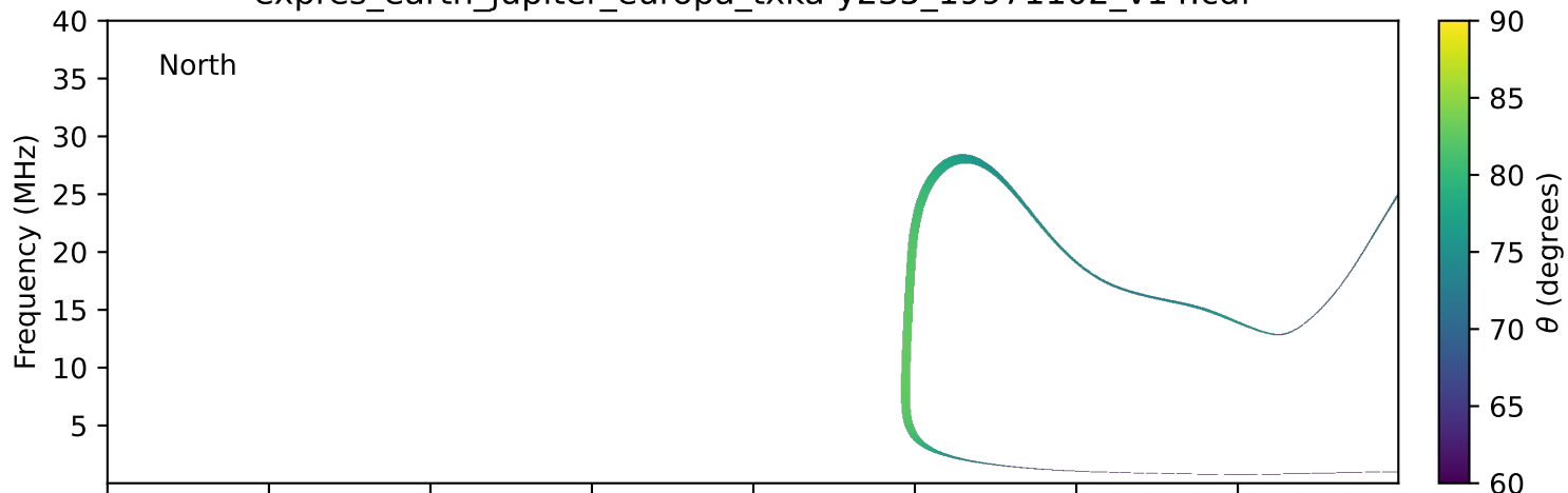
expres_earth_jupiter_europa_txka-y235_19971102_v14.cdf
