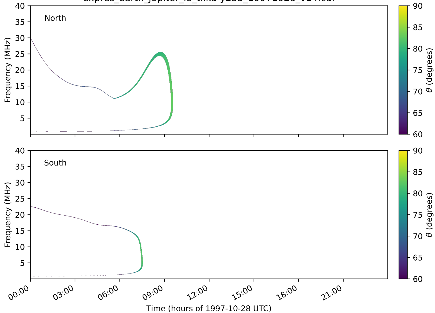
expres_earth_jupiter_io_txka-y235_19971028_v14.cdf
