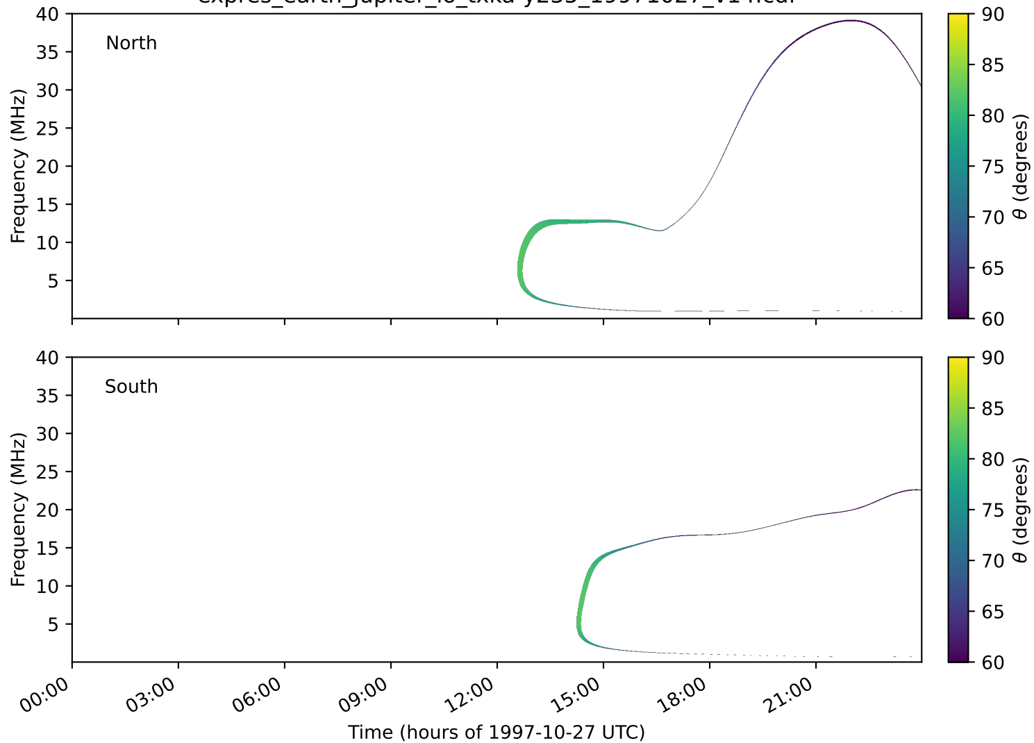
expres_earth_jupiter_io_txka-y235_19971027_v14.cdf
