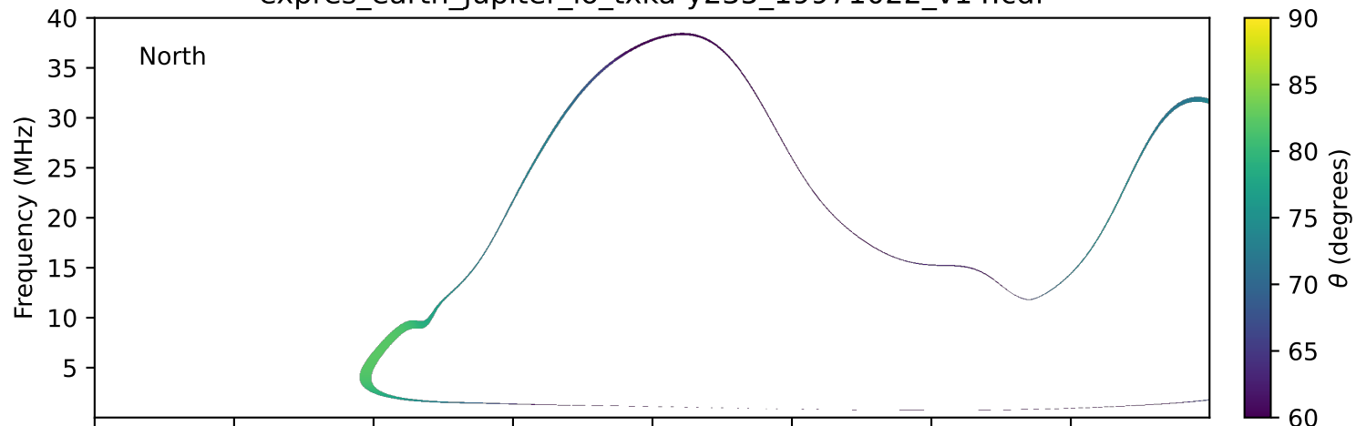
expres_earth_jupiter_io_txka-y235_19971022_v14.cdf
