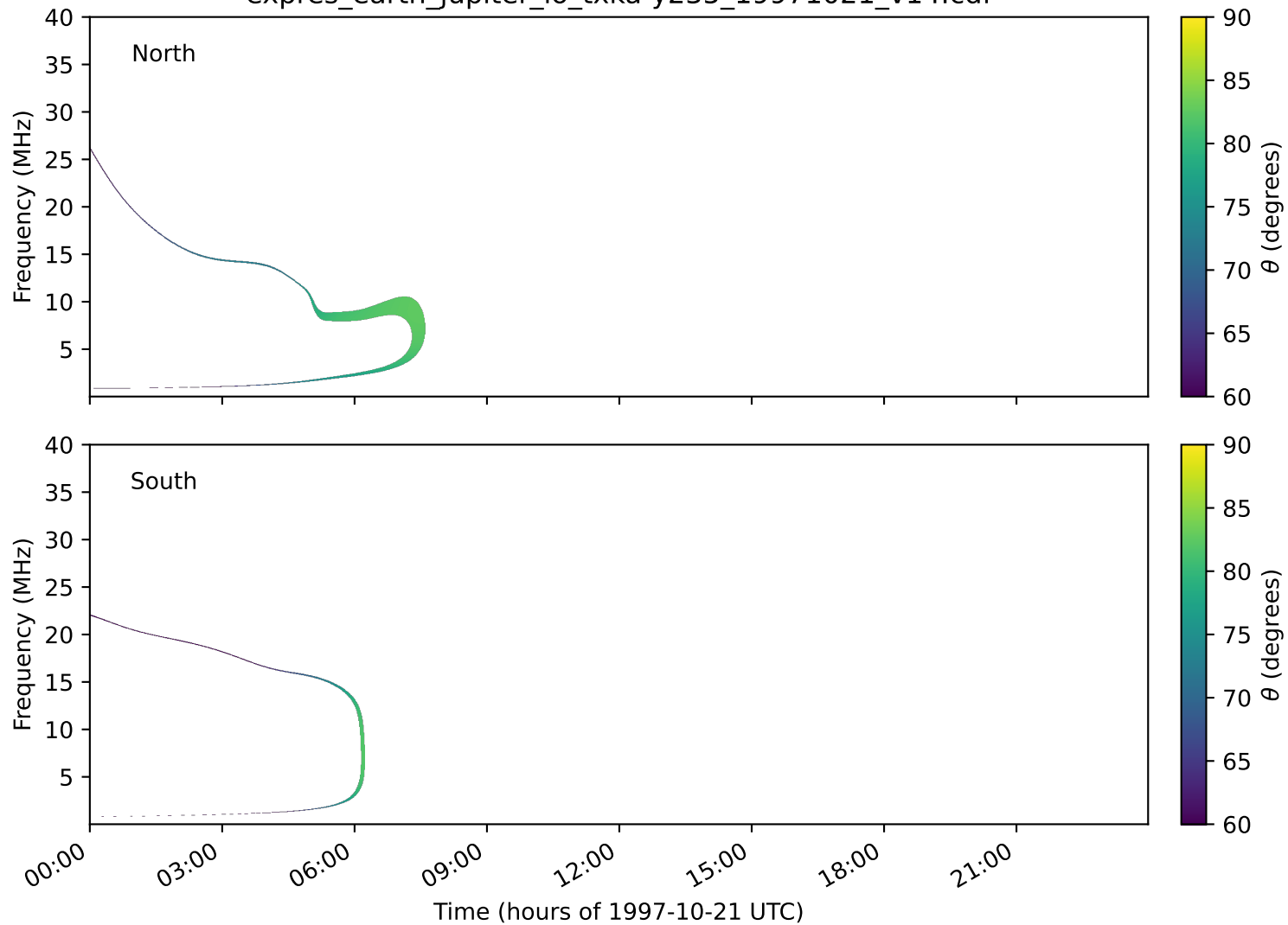
expres_earth_jupiter_io_txka-y235_19971021_v14.cdf
