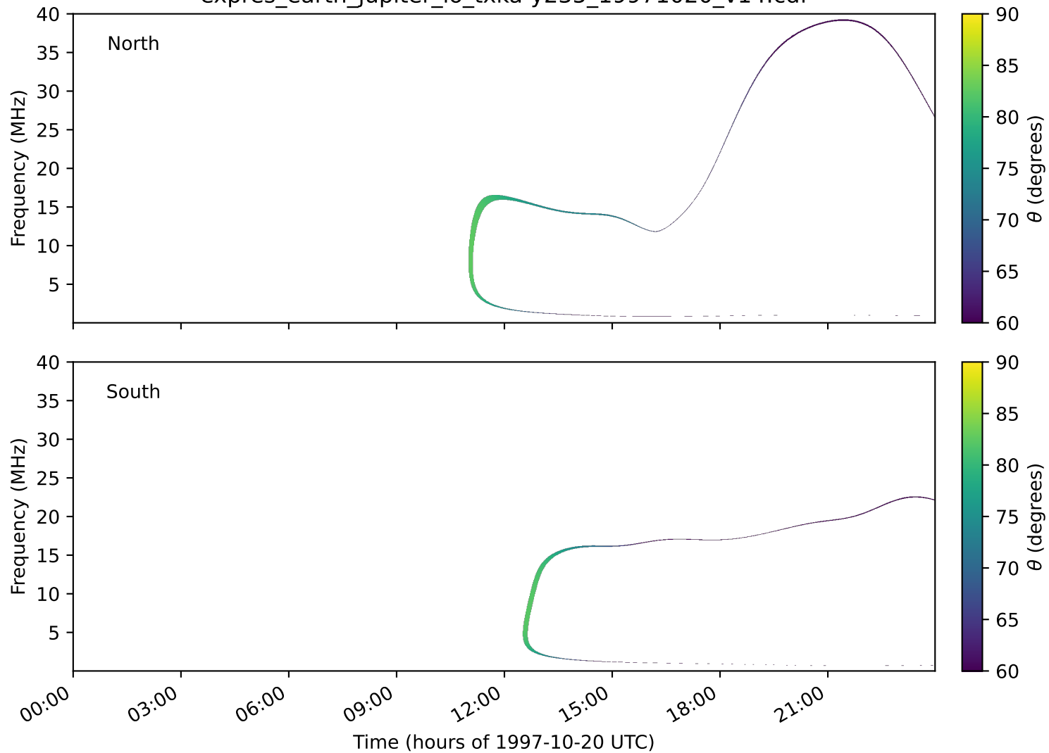
expres_earth_jupiter_io_txka-y235_19971020_v14.cdf
